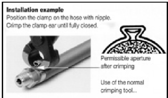
Pinched one-ear clamp and crimping tool
