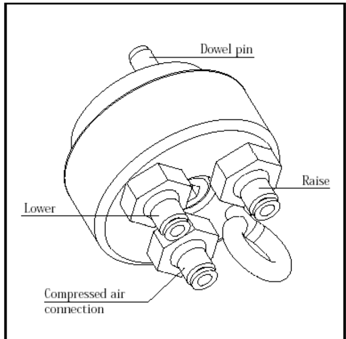
Hose adapter with nipples designation lift, lower
